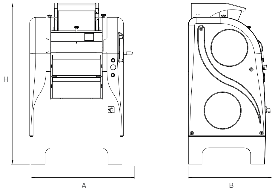
Technical drawings Refiner
